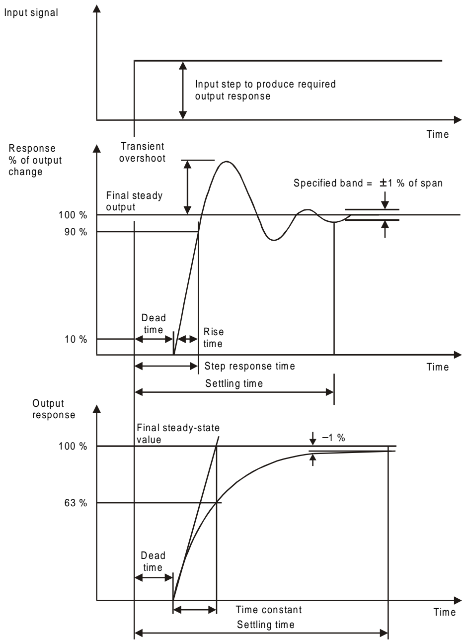
Figure 10 – Two examples of responses to a step input
