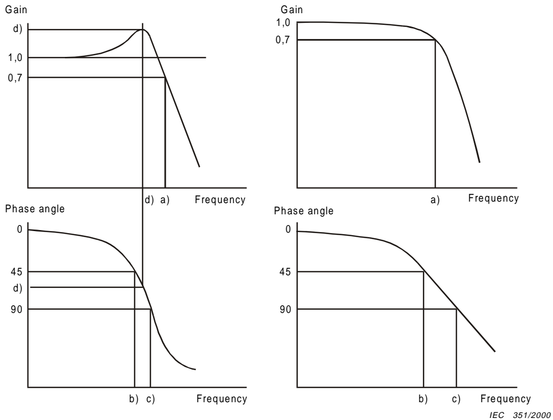
Figure 9 – Two examples of frequency response tests
