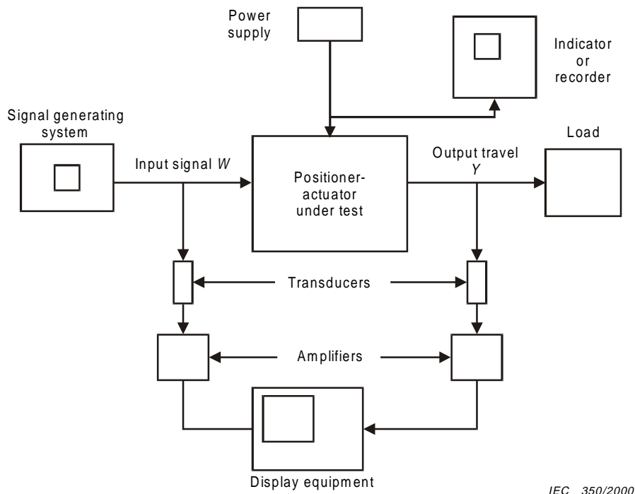
Figure 8 – Simple dynamic response test arrangement
