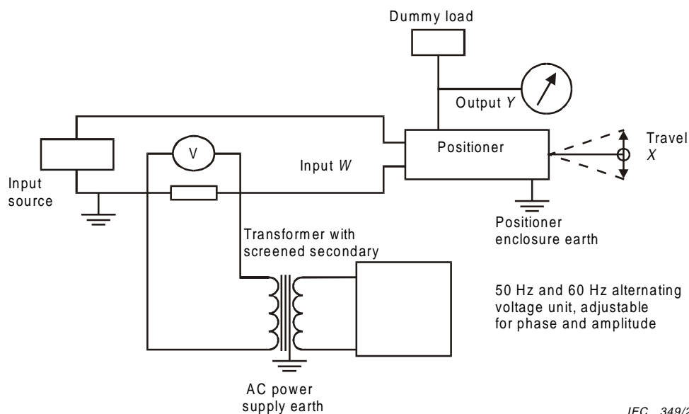
Figure 7 – Series mode interference
